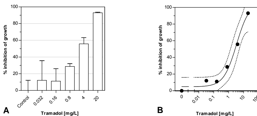
Figure 19: EC 50 estimation for tramadol based on % inhibition of number of animals. Average percent inhibition of growth (number of animals) \pm standard error; (A) Column graph, (B) log-scale graph; control (n=10), treatments (n=5); the dashed line marks the 95% confidence interval for the non-linear regression.
